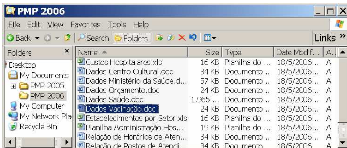
FIGURA 1 – Windows Explorer
